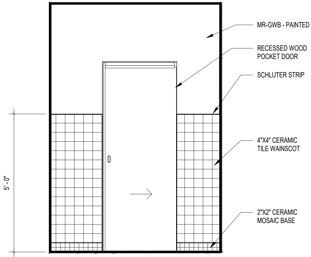
① LAUNDRY - EAST - AMENDED PERMIT 1/2" = 1'-0"
